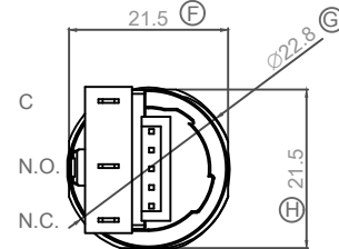
SWITCH
