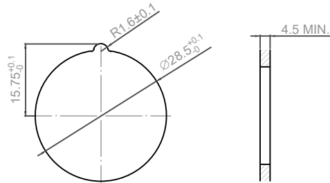
PANEL CUT OUT H=6.8
