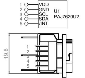
SENSOR
